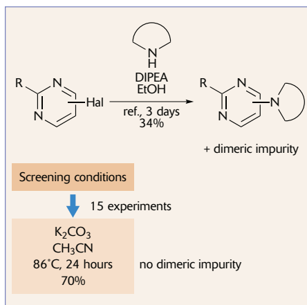
Figure 2 - DOE for the regioselective palladium-catalysed arylation of 4-chloropyrazole
